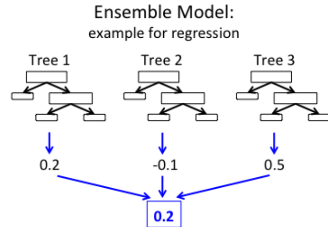
Gradient Boosting Tree
